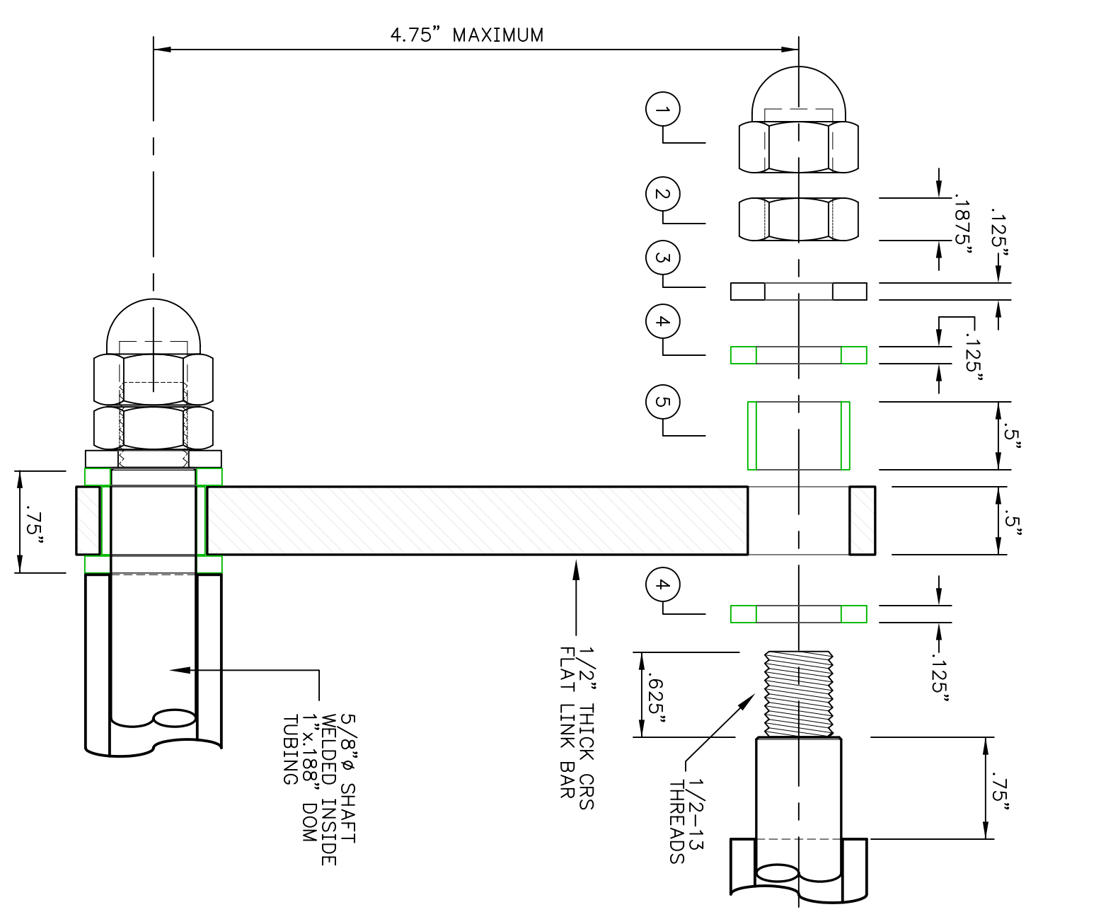
SCHEMATIC SECTIONAL VIEW
