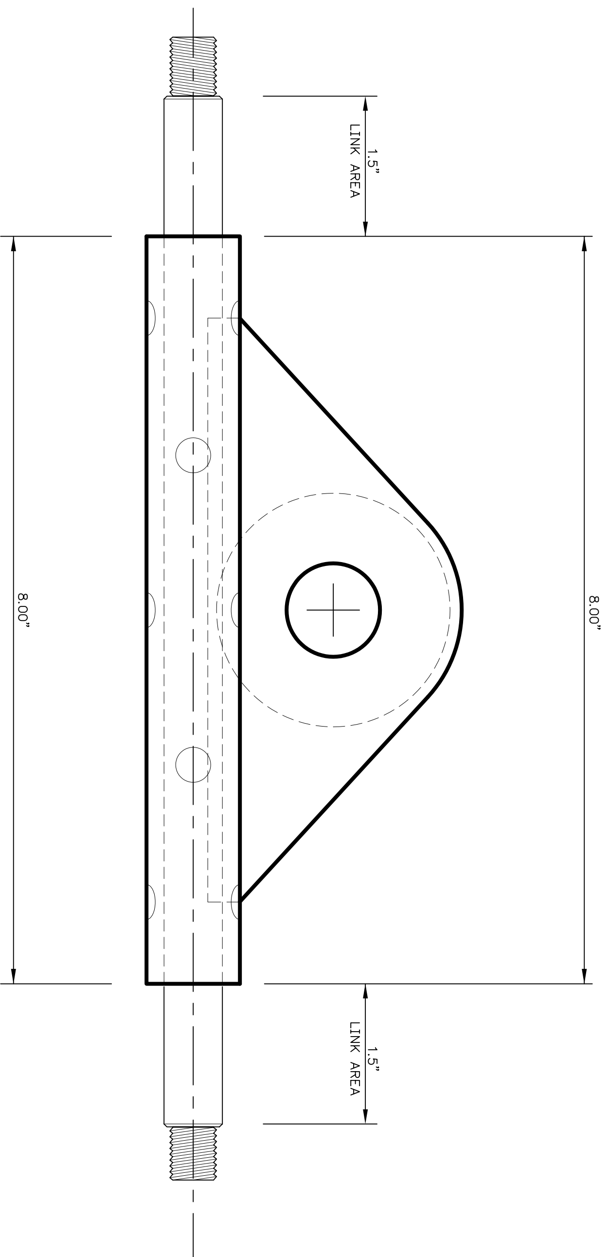
LOWER STEERING YOKE - TOP VIEW SCALE 1" = 1"
